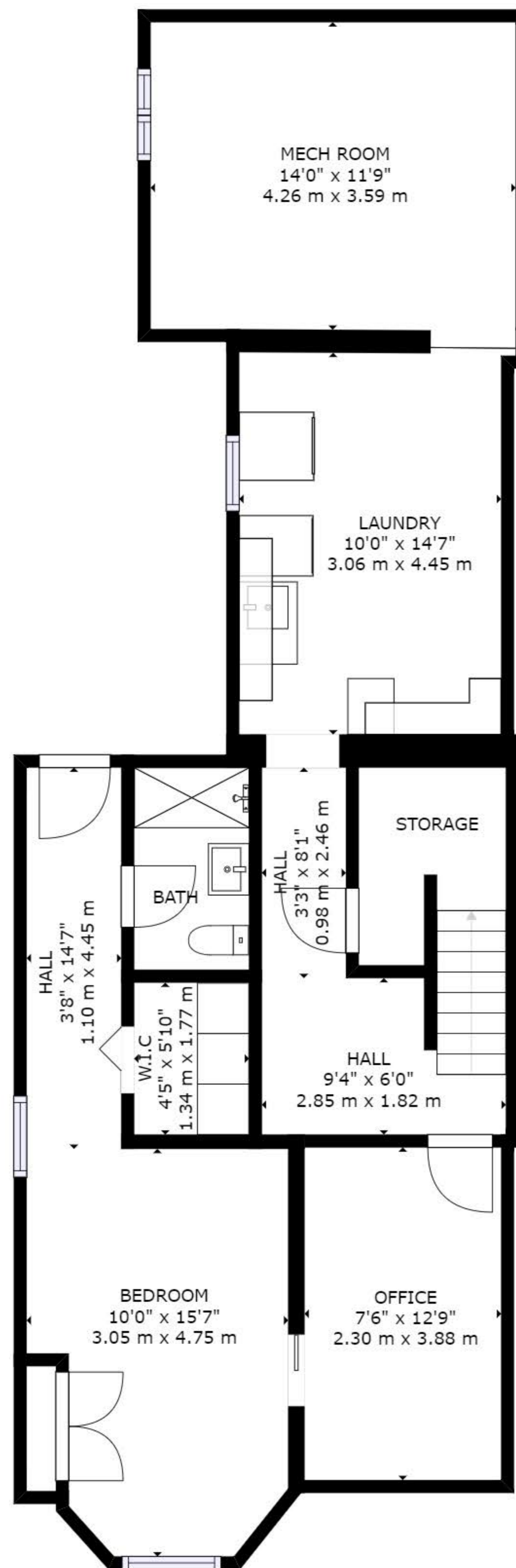
FLOOR 1
